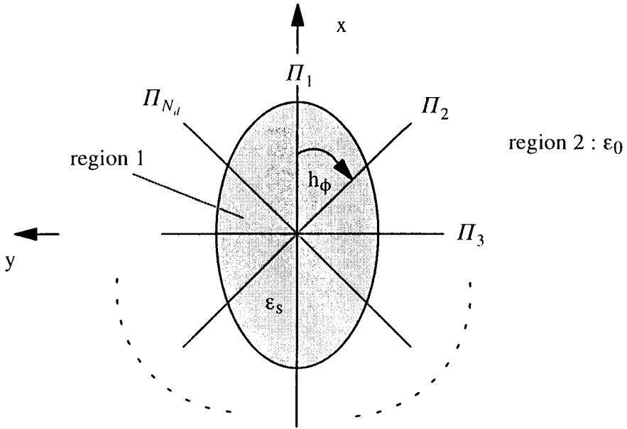
Figure 2. Equidistant discretization of the cylindrical cross-section taking periodicity into account.
