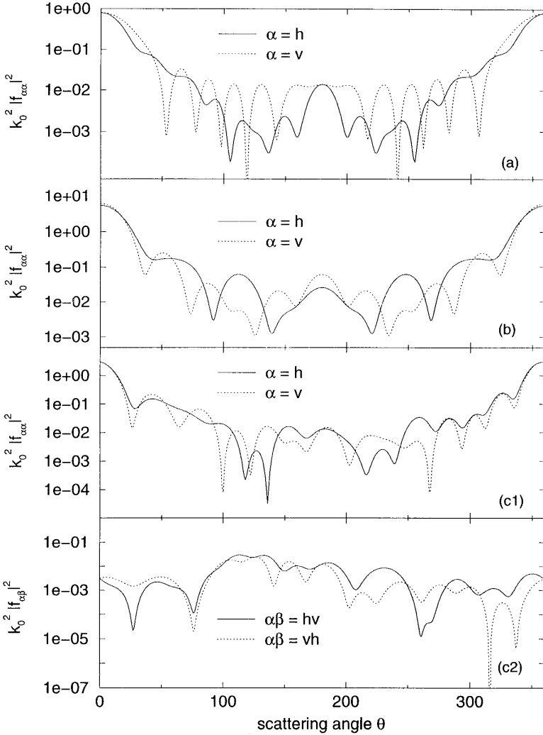
Figure 21. Differential scattering behavior of a prolate spheroid with a = 3 mm, b = 1.5 mm and \epsilon_s = 2.25 at f = 159.155 GHz ( k_0 a = 10 ). Independent of the orientation, the discretization parameters are N_d = 700 and ncut = 45 . (a) \Theta_p = \Phi_p = 0^\circ : \sigma_{ext} (DMF) = 0.518, \sigma_{ext} (B/H in [28]) = 0.519. (b) \Theta_p = \Phi_p = 90^\circ : \sigma_{ext} (DMF) = 1.645, \sigma_{ext} (B/H in [28]) = 1.647. (c1) \Theta_p = \Phi_p = 45^\circ : \sigma_{ext} (DMF) = 1.138, \sigma_{ext} (B/H in [28]) = 1.14. (c2) orientation as in (c1), but for hv - and vh -polarization.
