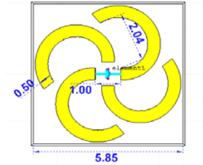
Figure 4. The structure of the absorber (all dimensions are in mm).
