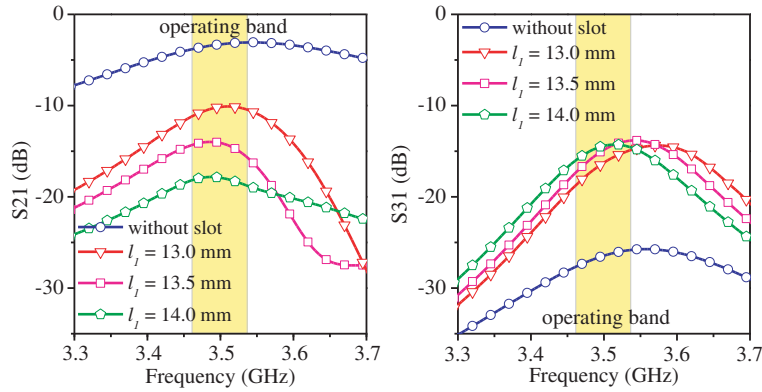
Figure 2. Effects of slot length on port isolation.
