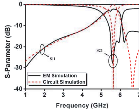
Figure 7. Simulated return loss of CBTR loaded microstrip line.
