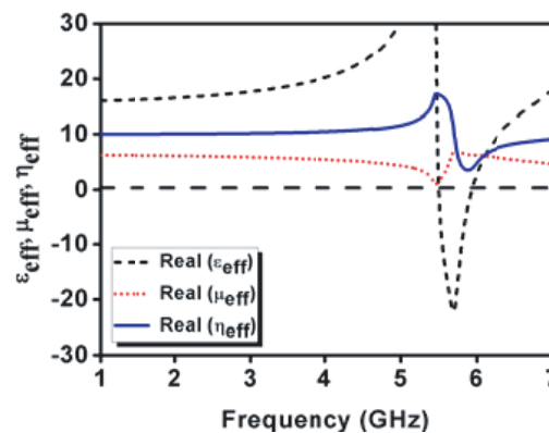
Figure 3. Effective permittivity ( \epsilon_{\text{eff}} ), permeability ( \mu_{\text{eff}} ) and refractive index ( \eta_{\text{eff}} ) of proposed unit cell.
