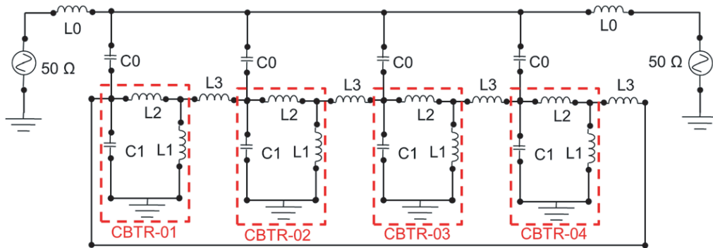
Figure 6. Equivalent circuit model of CBTRs loaded microstrip line.
