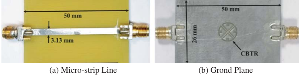
Figure 4. The fabricated proto of CBTR loaded microstrip line.
