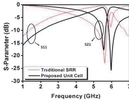
Figure 2. Comparison between traditional SRR and proposed unit cell.
