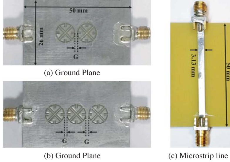
Figure 8. Fabricated prototype for (a) N = 2 , (b) N = 3 , (c) microstrip line.
