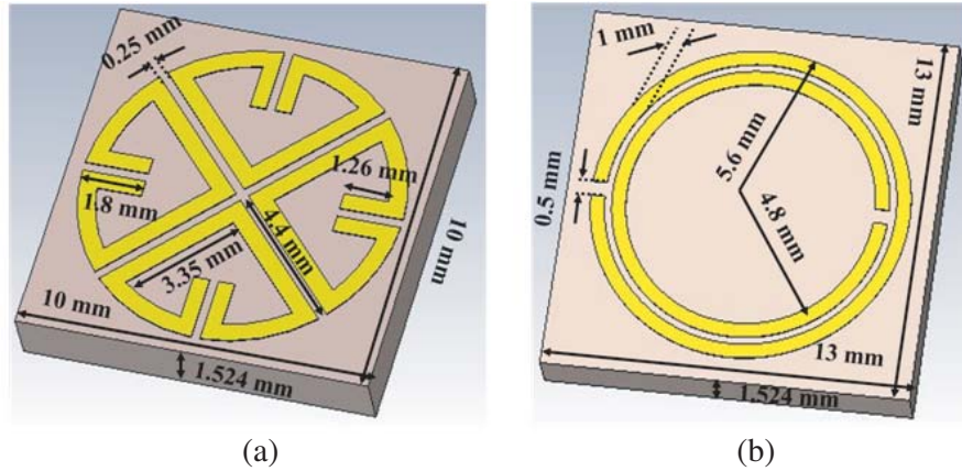
Figure 1. Geometry of (a) proposed unit cell, (b) traditional SRR.
