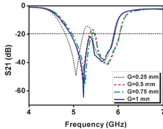
Figure 10. Variation in S_{21} (dB) with the change in gap ( G ).
