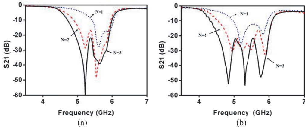
Figure 9. (a) Simulated and (b) measured S_{21} (dB) of CBTRs loaded microstrip line with increasing order.
