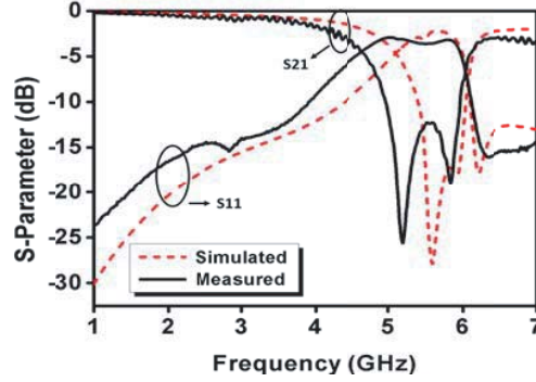
Figure 5. S -parameter result of CBTR loaded microstrip line.
