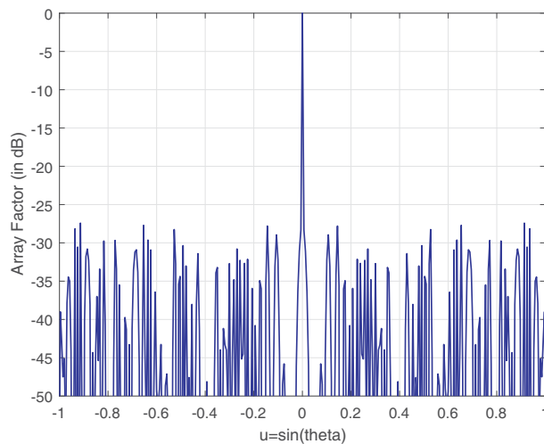
Figure 9. Asymmetrical thinned linear array with fill factor of 45%.
