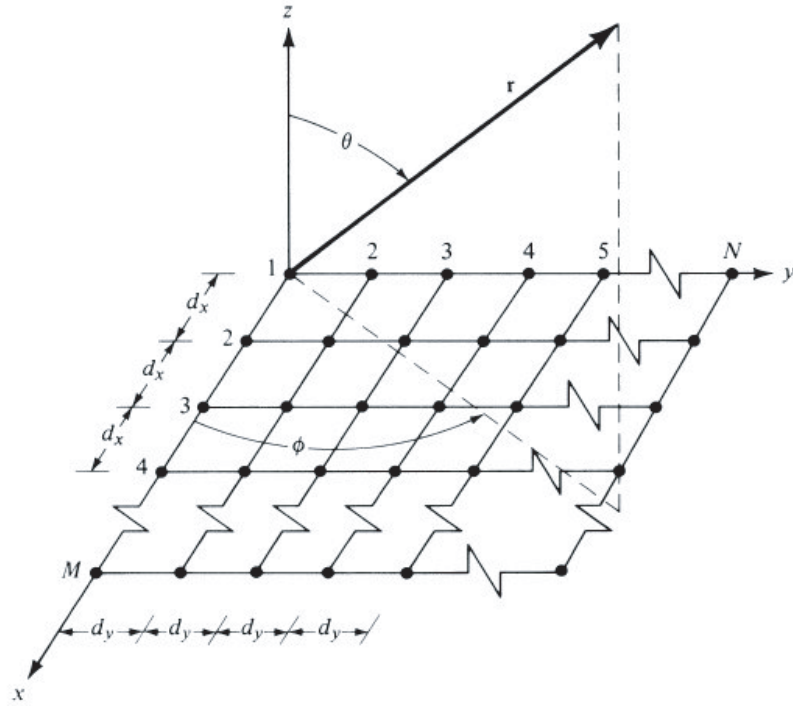
Figure 11. Arrangement of planar grid of antenna element.
