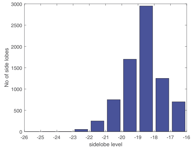
Figure 8. Count of side lobes (10000 trials) by histogram representation.
