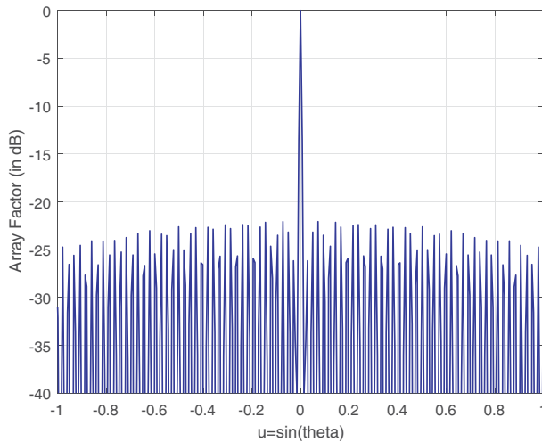
Figure 1. Symmetrical thinned linear array with fill factor of 77%.
