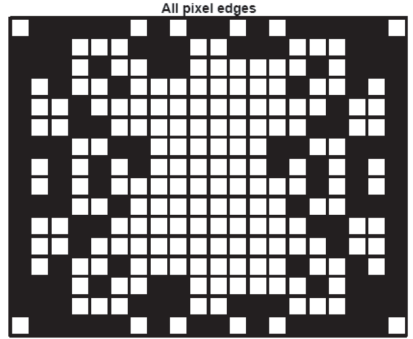
Figure 15. Contour of thinned planar array with a fill factor of 55%.
