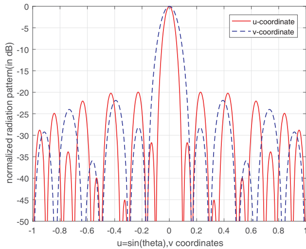
Figure 12. U-V section diagram of planar array without thinning.
