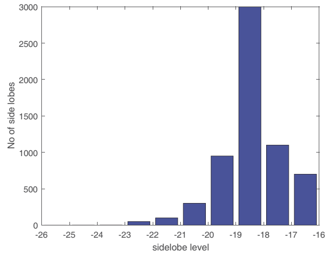
Figure 2. Count of side lobes (10000 trials) by histogram representation.
