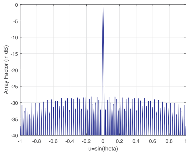
Figure 5. Symmetrical thinned linear array with fill factor of 45%.
