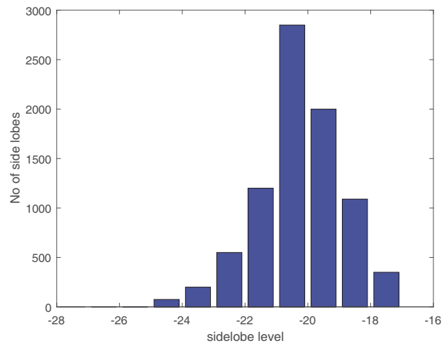
Figure 6. Count of side lobes (10000 trials) by histogram representation.
