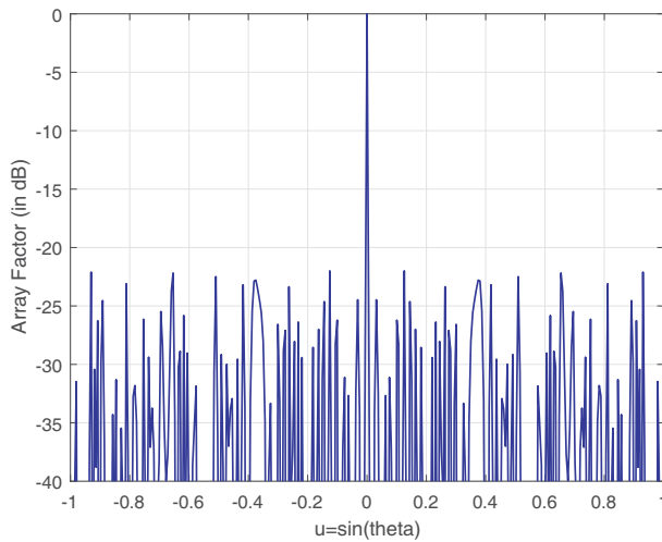
Figure 7. Asymmetrical thinned linear array with fill factor of 71.80%.
