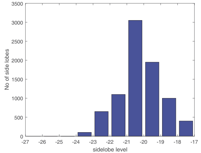
Figure 4. Count of side lobes (10000 trials) by histogram representation.
