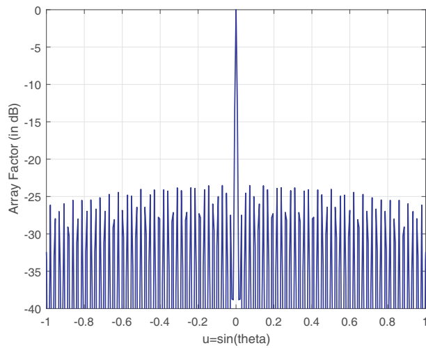
Figure 3. Symmetrical thinned linear array with fill factor of 63%.
