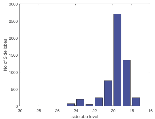
Figure 10. Count of side lobes (10000 trials) by histogram representation.
