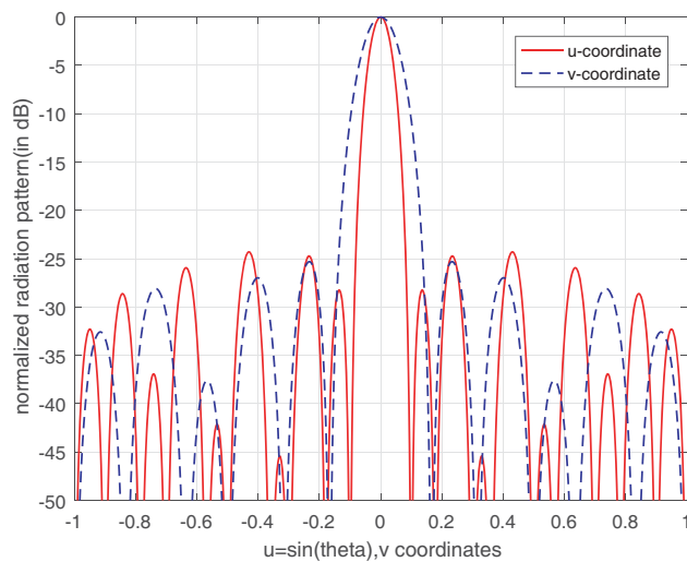
Figure 16. U-V section diagram of thinned planar array with fill factor 45%.
