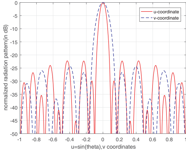
Figure 14. U-V section diagram of thinned planar array with fill factor 55%.
