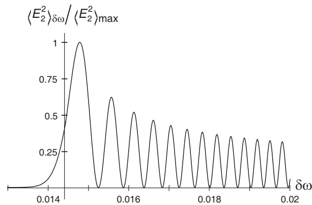
Figure 1. Plasma line spectrum versus relative frequency shift \delta\omega = (\omega - \omega_{p0}) / \omega_{p0} . The plasma line intensity is normalized to its maximum value.
