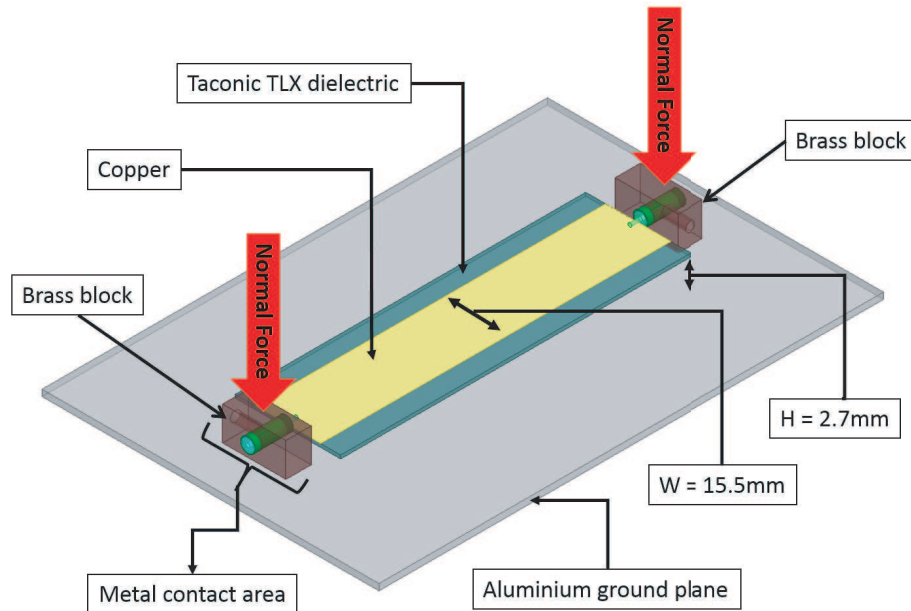
Figure 1. Test setup synoptic.
