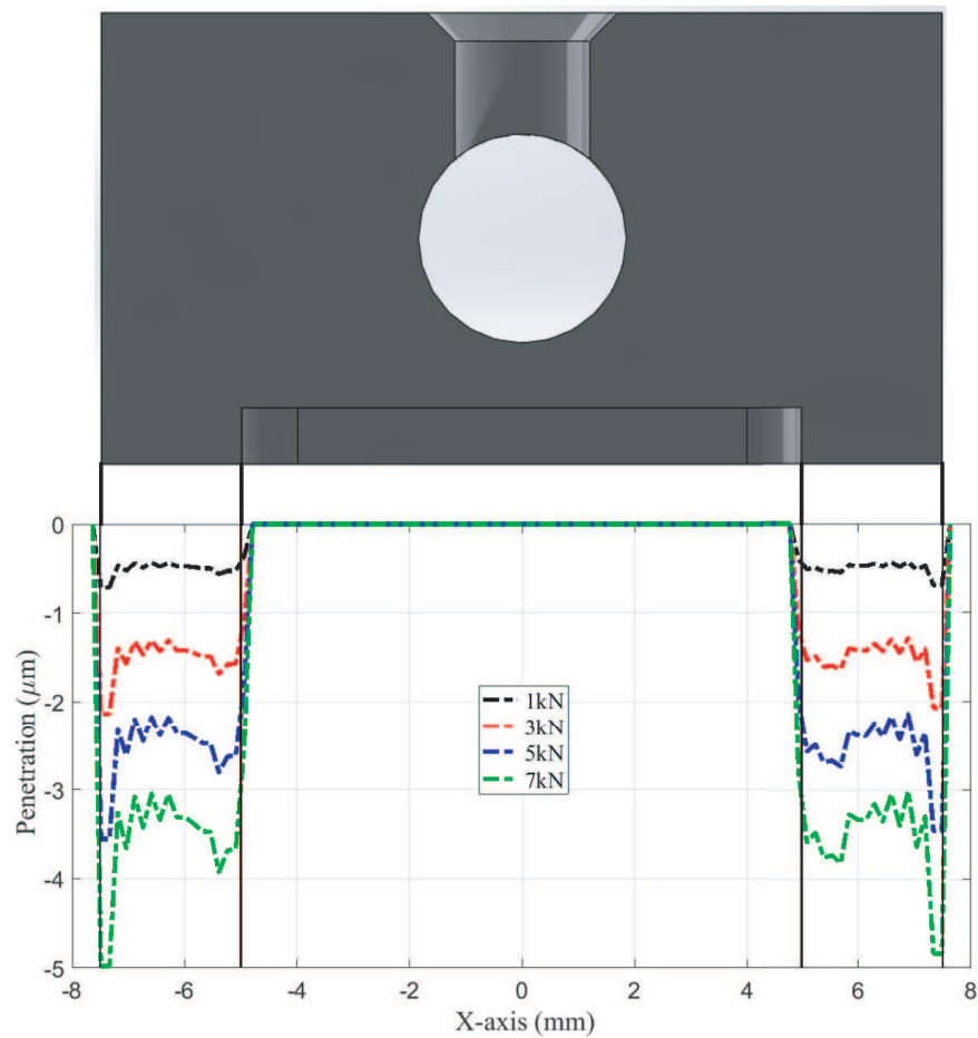
Figure 3. Penetration evolution versus normal force for hollowed-out profile (cross-sectional view).
