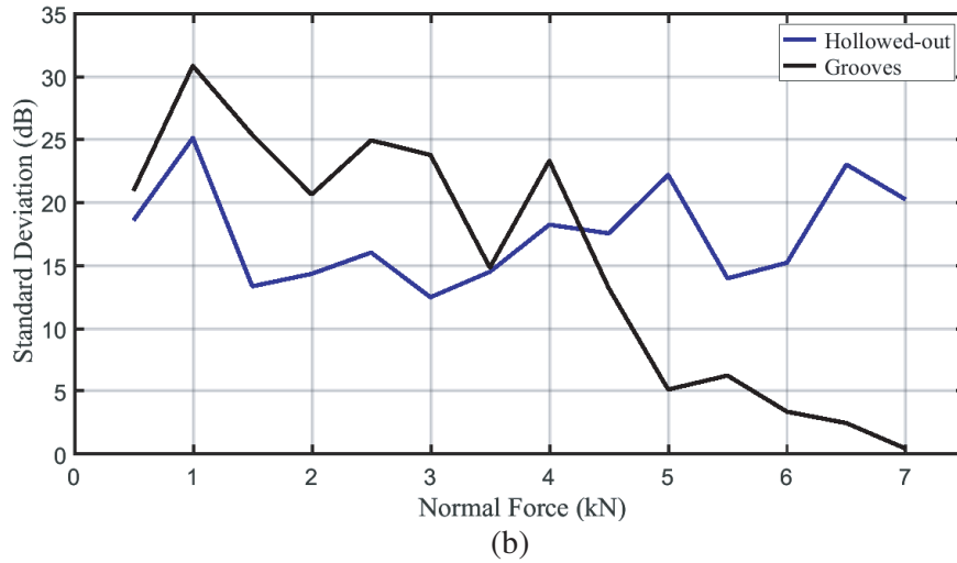
Figure 6. Comparison between hollowed-out and grooves surface profile of PIM measurements as a function of normal force for 45 \text{ mm}^2 contact area. (a) Average and 68% confidence interval. (b) Standard deviation.
