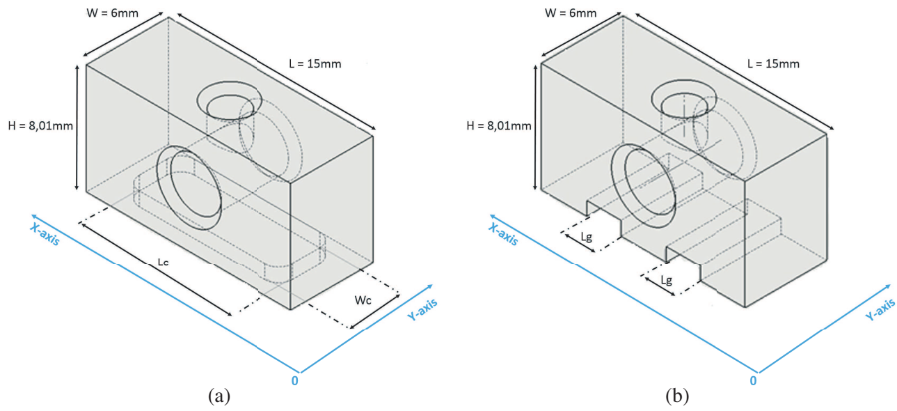
Figure 2. Mechanical design of (a) hollowed-out brass block, (b) grooves brass block.
