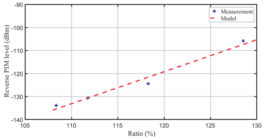
Figure 7. Average PIM level at 7 kN in function of the ratio between penetration and contact areas.
