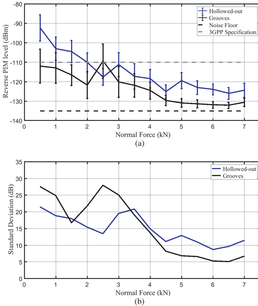
Figure 5. Comparison between hollowed-out and grooves surface profile of PIM measurements as a function of normal force for 60 mm 2 contact area. (a) Average and 68% confidence interval. (b) Standard deviation.
