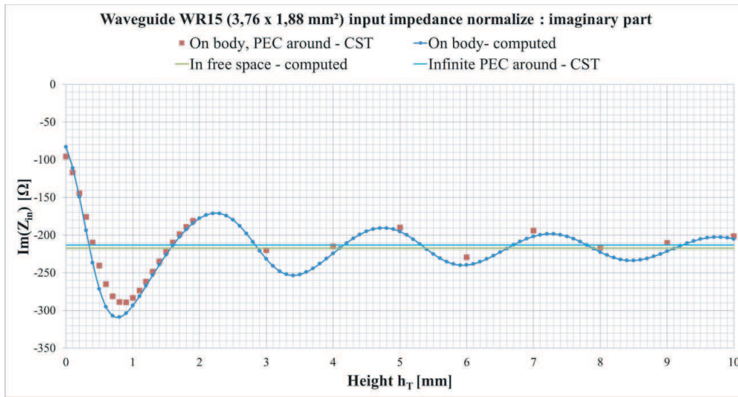
Figure 6. Computed and simulated input impedance imaginary part variation along the height h_T at 60 GHz.
