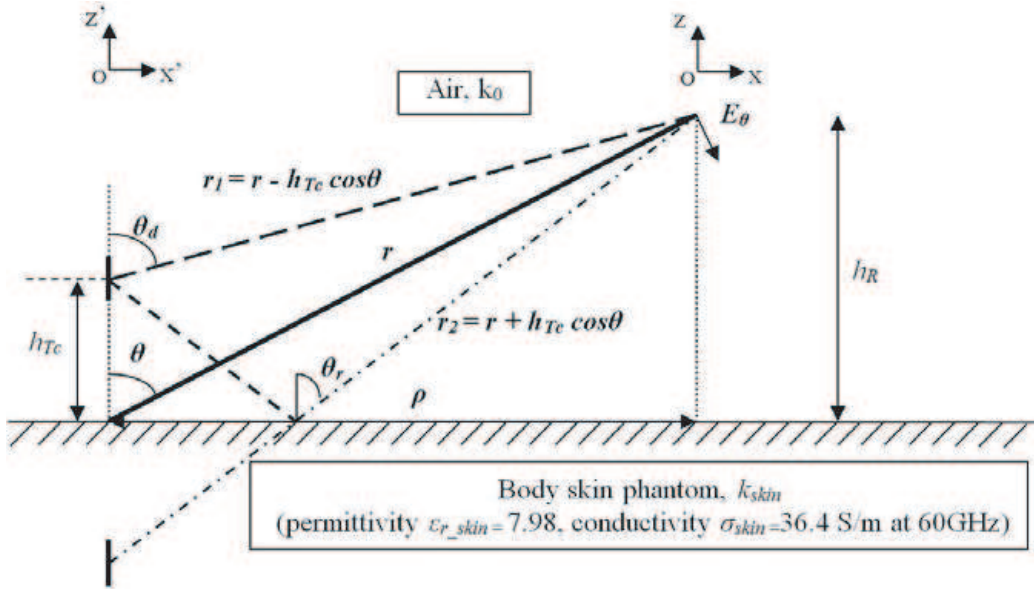
Figure 1. Vertical electric dipole in air at height h_{Tc} over a planar body skin phantom.
