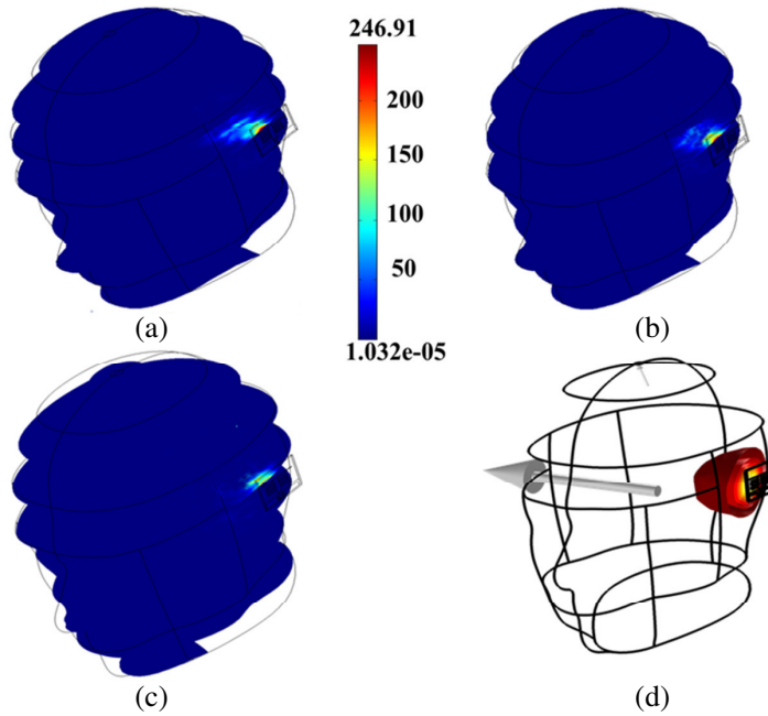
Figure 7. SAR plots in COMSOL multiphysics for (a) plane ground, (b) inverted U-shape ground, (c) truncated ground plane, (d) direction of heat flux plot of the final antenna.
