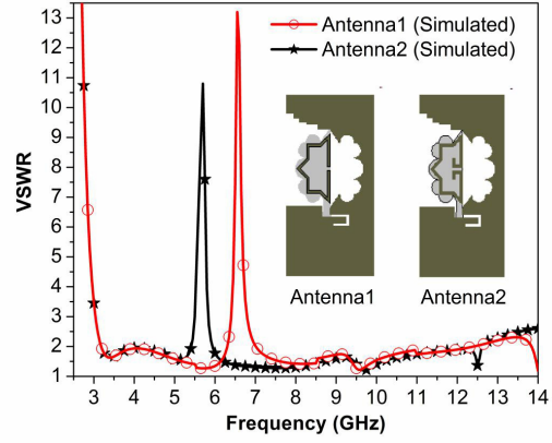
Figure 4. Comparison between Antenna 1 and the Antenna 2 (loaded with L-stub) ( w_4 = 4.8 mm).
