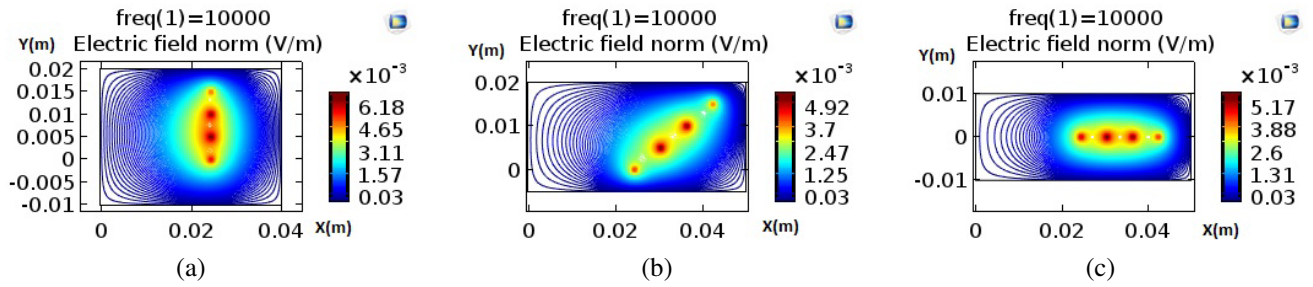
Figure 4. Electric field norm at 10 kHz (V/m) in (a) Helical. (b) Conical. (c) Circular.
