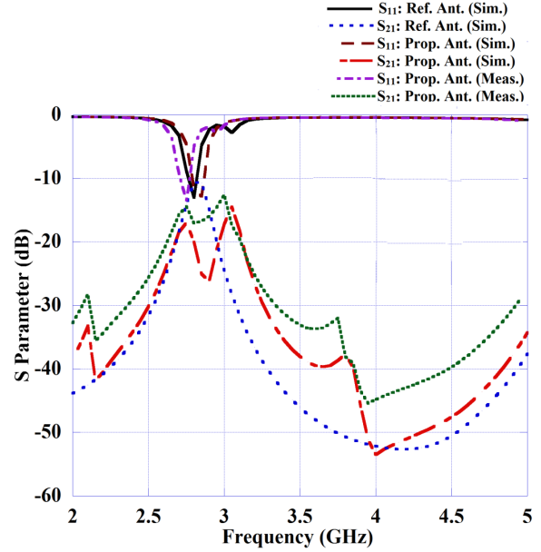
Figure 4. S parameters ( S_{11} & S_{21} ) of the antenna elements.
