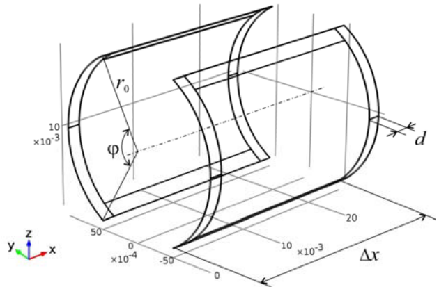
Figure 2. 3D image of a geometrical model of a saddle-shaped coil in COMSOL Multiphysics.
