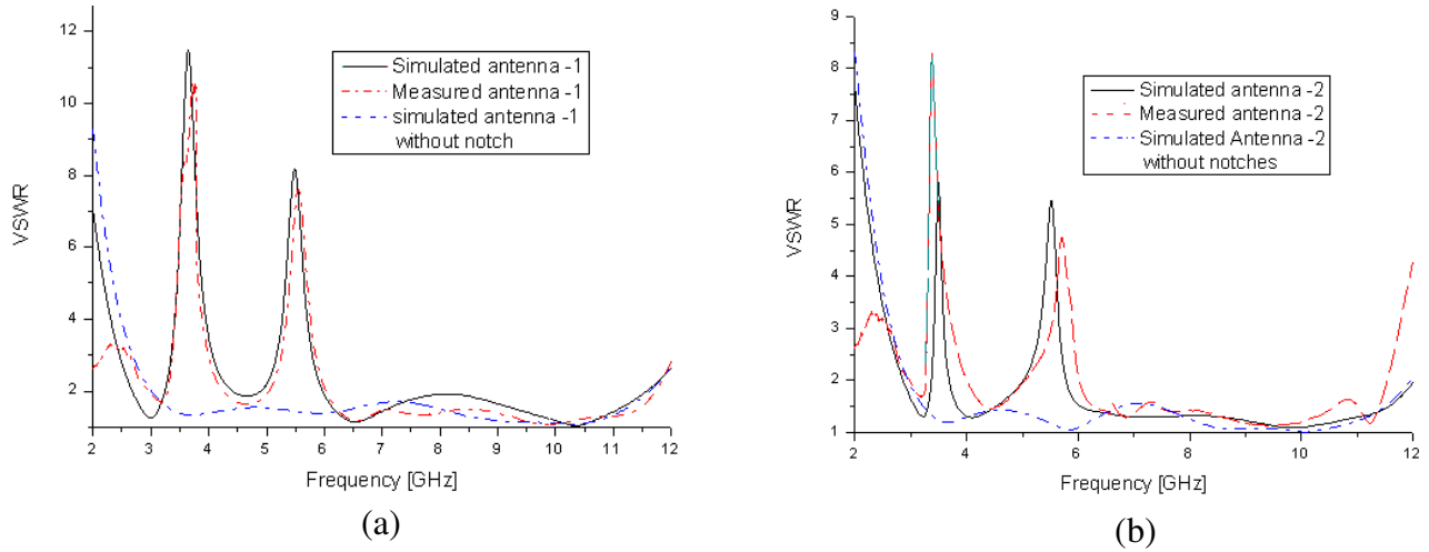
Figure 5. VSWR versus frequency curve: (a) Antenna-1 with symmetrical ground plane; (b) Antenna-2 with asymmetrical ground plane.
