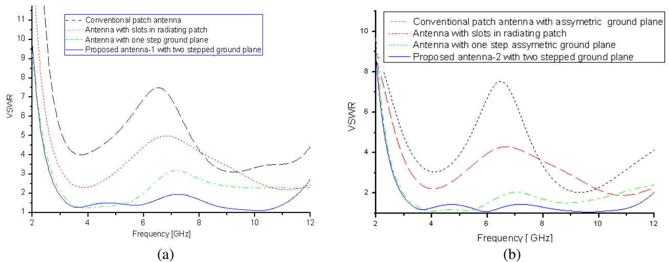
Figure 4. VSWR versus frequency curves for: (a) Antennas 3(a)–(d) with symmetrical ground plane; (b) Antennas 3(e)–(h) with asymmetrical ground plane.
