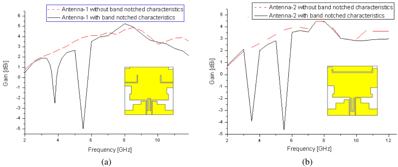
Figure 12. Gain versus frequency curves: (a) Antenna-1; (b) Antenna-2.
