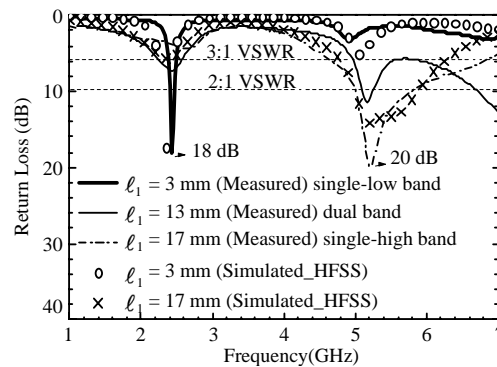
Figure 4. The return loss of the proposed antenna design for the parameter- \ell_1 variation.
