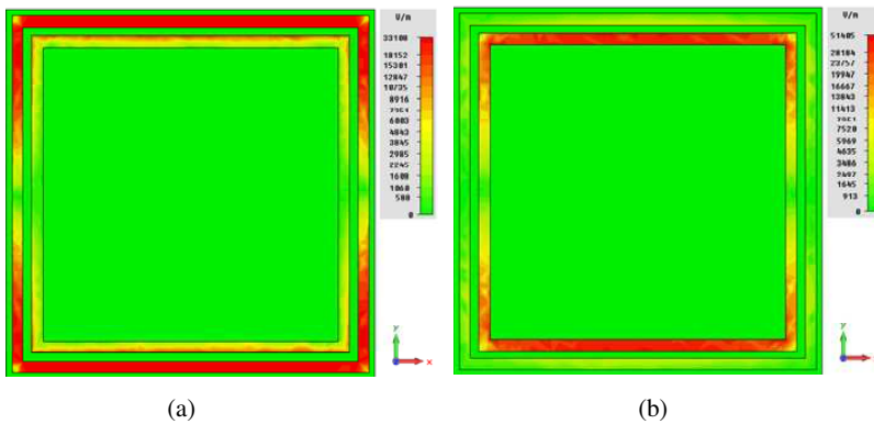
Figure 3. Electric field distribution diagrams at two different frequencies. (a) 1.73 GHz. (b) 2.64 GHz.
