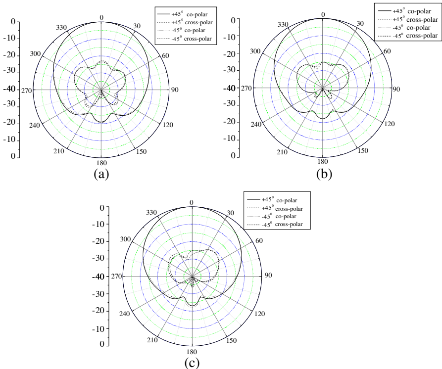
Figure 8. Measured H -plane radiation pattern for \pm 45^\circ polarization. (a) 1.71 GHz. (b) 1.94 GHz. (c) 2.17 GHz.
