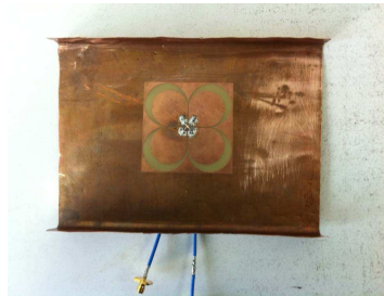
Figure 2. Photo of the fabricated antenna element.
