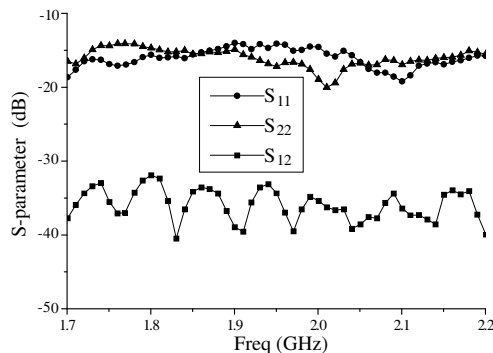
Figure 3. Measured return loss and isolation.
