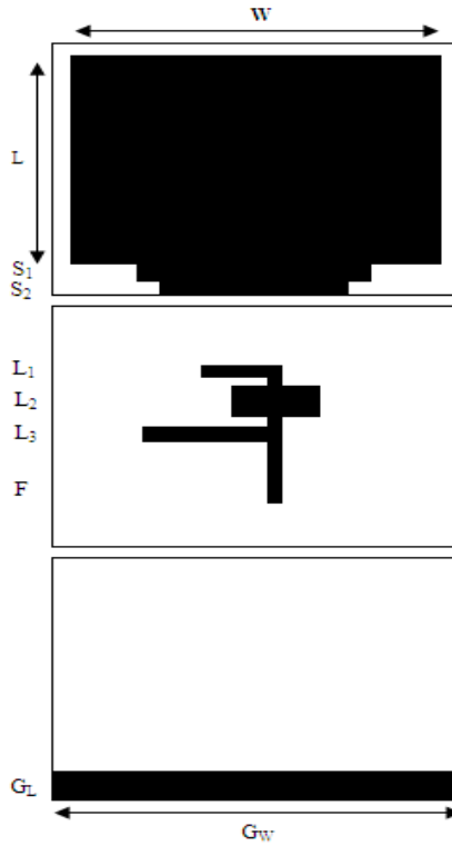
Figure 1. Basic configuration of stepped patch antenna with Pi matching network and partial ground.
