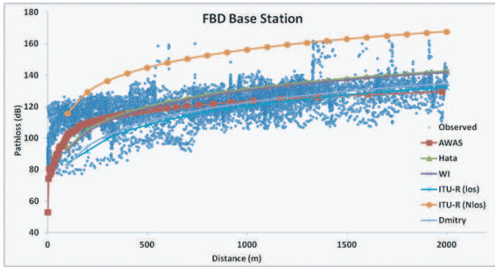
Figure 7. Comparison of observed path loss values with various models for FBD base station.
