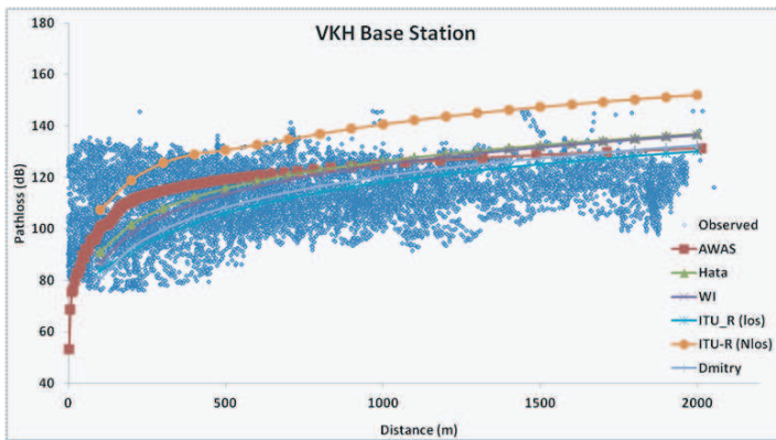
Figure 8. Comparison of observed path loss values with various models for VKH base station.
