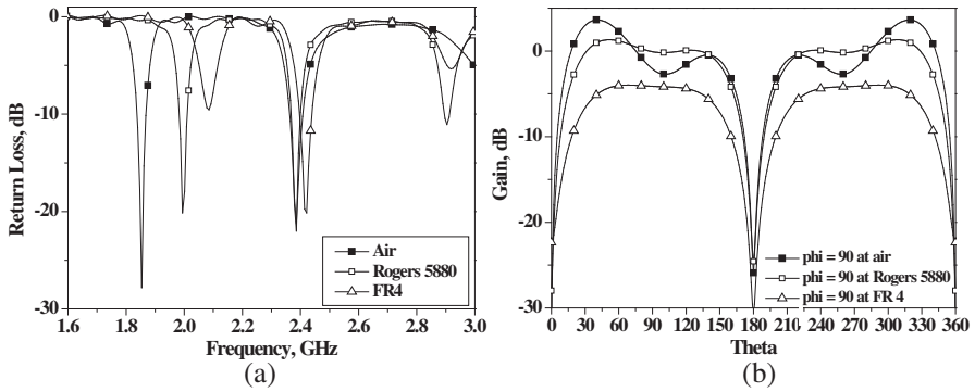
Figure 5. Frequency response and antenna gain VS. different \epsilon_r . (a) Return loss. (b) Radiation pattern at the ZOR VS. the elevation angle: Parameters are \text{via}_r = 0.4 \text{ mm} , the number of the \text{vias}_s = 8 , R_d = 0.1 \text{ mm} .
