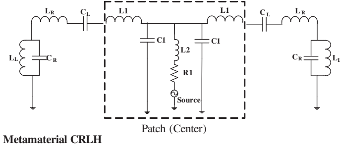
Figure 2. Equivalent circuit of the proposed CRLH microstrip antenna.
