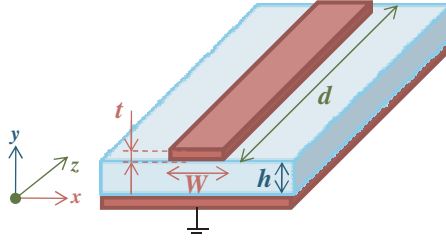
Figure 2. Geometrical representation of microstrip TL.
