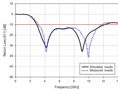
Figure 7. Simulated and measured return loss results of antenna #1 design.
