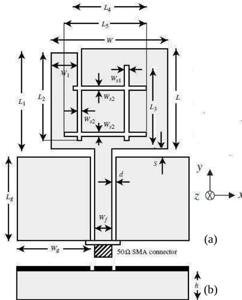
Figure 1. Geometry of the proposed antenna. (a) Top view, (b) front view.
