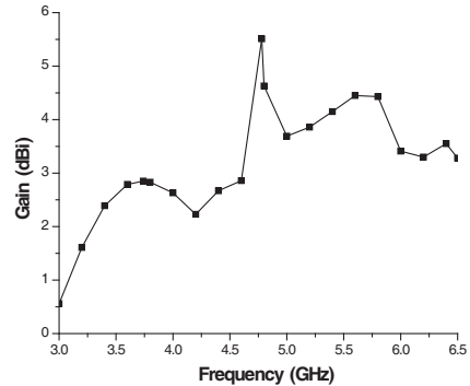
Figure 4. Simulated gain variation of the antenna against frequency.
