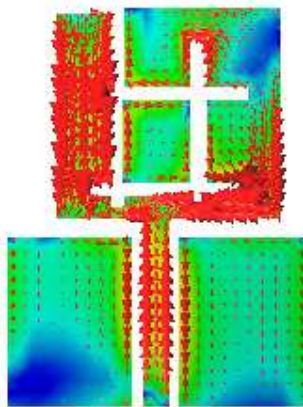
Figure 9. Current distributions at 5.42 GHz.
