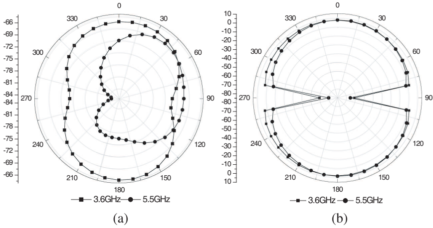
Figure 10. Radiation pattern plot of proposed antenna. (a) Azimuthal plane, (b) elevation plane.
