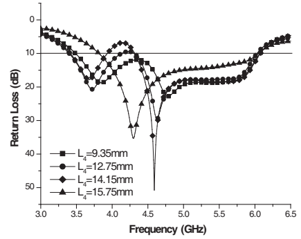
Figure 6. Effect of variation of slot length L_4 on return loss.
