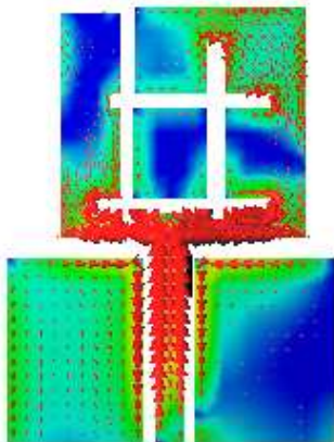
Figure 8. Current distributions at 3.74 GHz.
