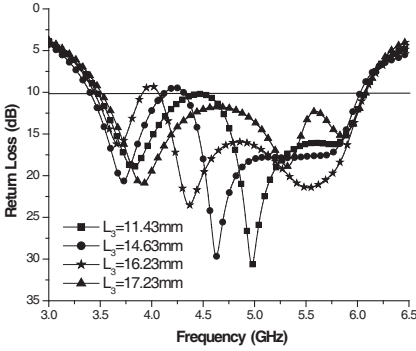
Figure 5. Effect of variation of slot length L_3 on return loss.
