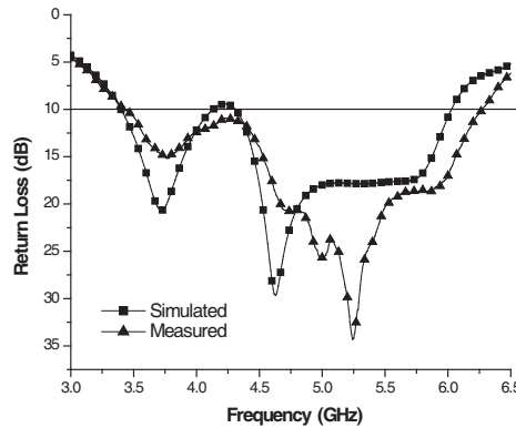
Figure 11. Simulated and measured return-losses of proposed antenna.
