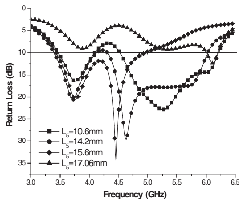
Figure 7. Effect of variation of slot length L_5 on return loss.
