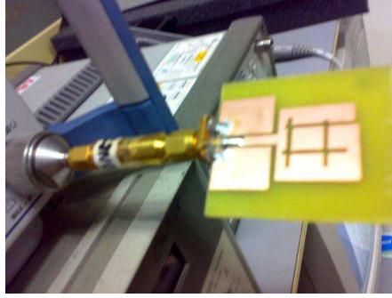
Figure 2. Fabricated antennas with proposed design.
