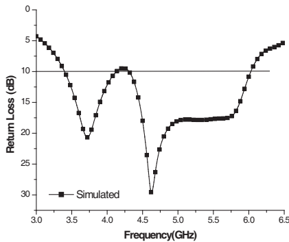
Figure 3. Simulated return-loss of proposed antenna.
