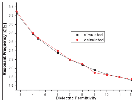
Figure 5. Calculated and simulated resonant frequency of the miniaturized FSS for different permittivity.
