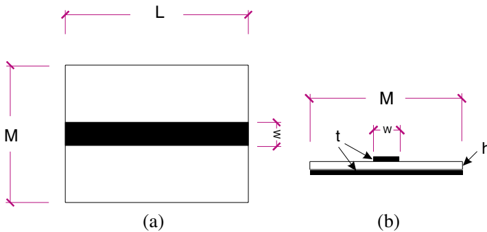
Figure 1. Geometry of the MUT samples: (a) Top view; (b) side view.
