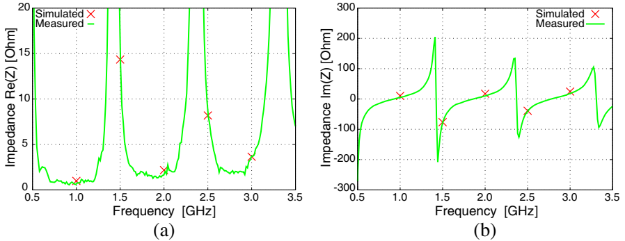
Figure 4. FR4 . Comparison between simulated and measured impedance values of (a) \text{Re}\{Z\} and (b) \text{Im}\{Z\} .
