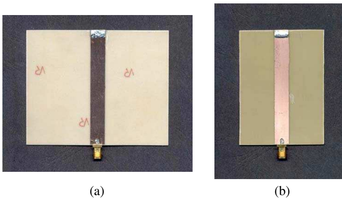
Figure 2. MUT samples: (a) FR4 and (b) Arlon substrates.
