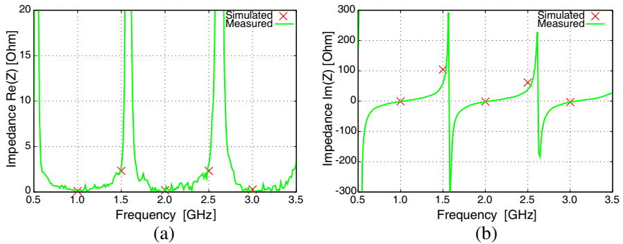
Figure 5. Arlon . Comparison between simulated and measured impedance values of (a) \text{Re}\{Z\} and (b) \text{Im}\{Z\} .
