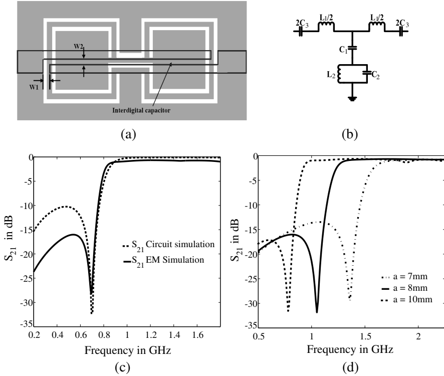
Figure 3. Highpass filter. (a) Geometry. (b) Equivalent circuit. (c) Insertion loss. (d) Transmission response for various 'a'.
