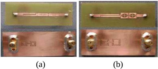
Figure 5. Fabricated proposed BPFs. (a) Type 1. (b) Type 2.
