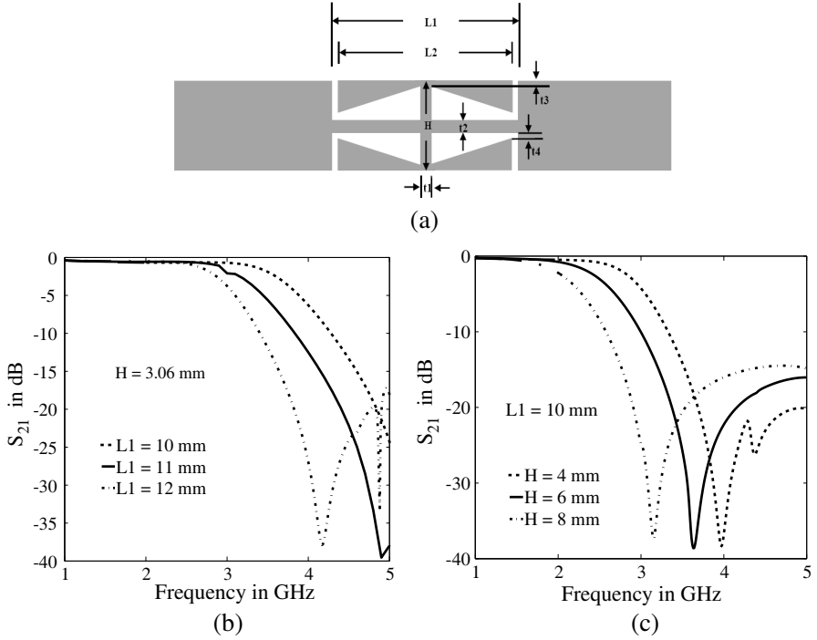
Figure 4. (a) Geometry of single CMRC. (b) Frequency response for various lengths. (c) Frequency response for various widths.
