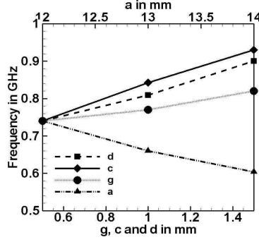
Figure 2. Variation of resonance frequency vs dimensions of OSSRR. (Side length varied from 12–14 mm and c , g , d varied from 0.5–1.5 mm.)
