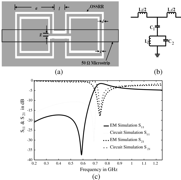
Figure 1. Open slot split ring resonator DGS. (a) Geometry. (b) Equivalent circuit. (c) Simulated scattering parameters of OSSRR.
