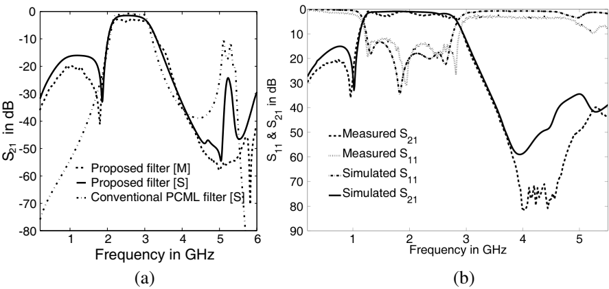
Figure 6. Scattering parameters of proposed BPFs. (a) Type 1. (b) Type 2. (M→ measurement, S→ simulation.)
