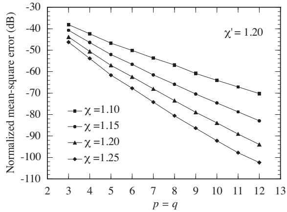
Figure 8. Helicoidal scanning. Mean-square reconstruction error of V .
