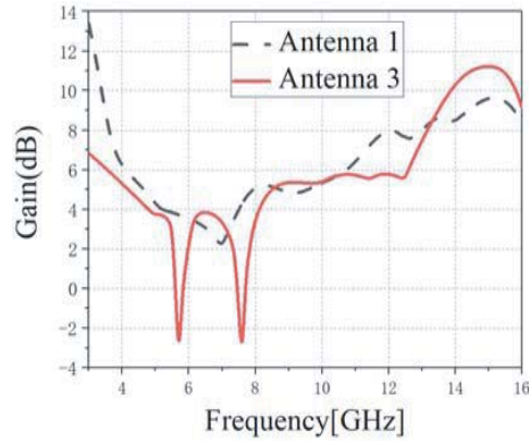
Figure 8. Gain of the proposed antenna.
