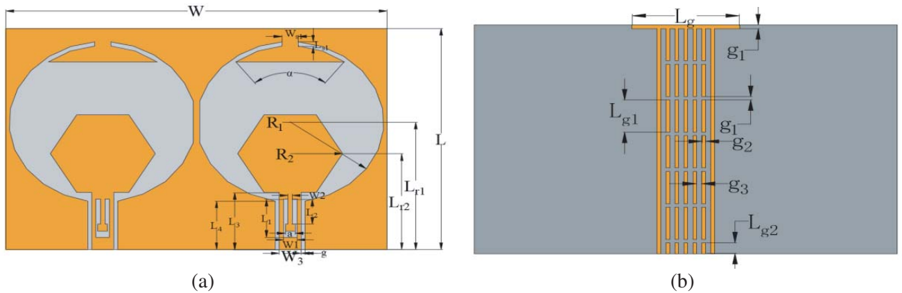
Figure 1. Geometry of the proposed antenna. (a) Top view. (b) Bottom view.
