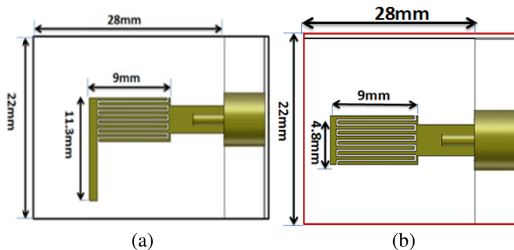
Figure 3. The layout of Unit cell CRLH antenna. (a) With stub. (b) With stub-less.
