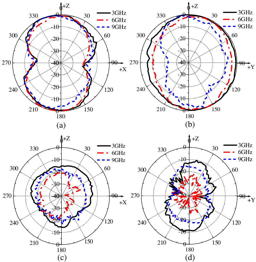
Figure 7. Measured co-polarization and cross-polarization radiation patterns (Unit: dBi). (a) Co-polarization component in E -plane, (b) co-polarization component in H -plane, (c) cross-polarization component in E -plane, (d) cross-polarization component in H -plane.
